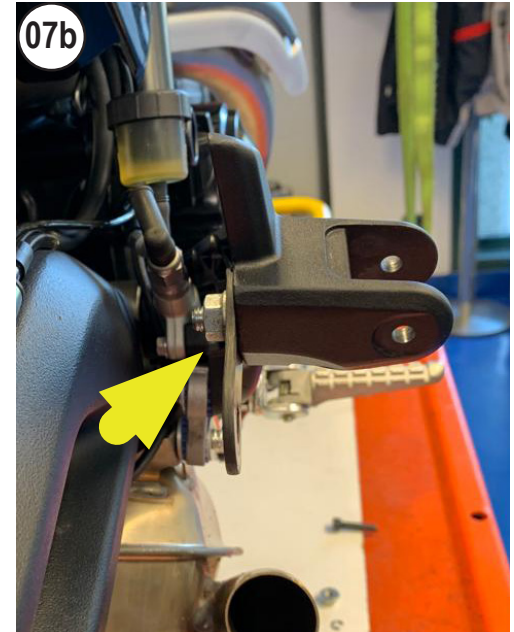
FASTENERS STACKING
