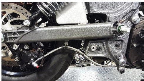
Fig.1.25 bracket removed
