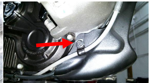
Fig. 2.23 install screw right side
